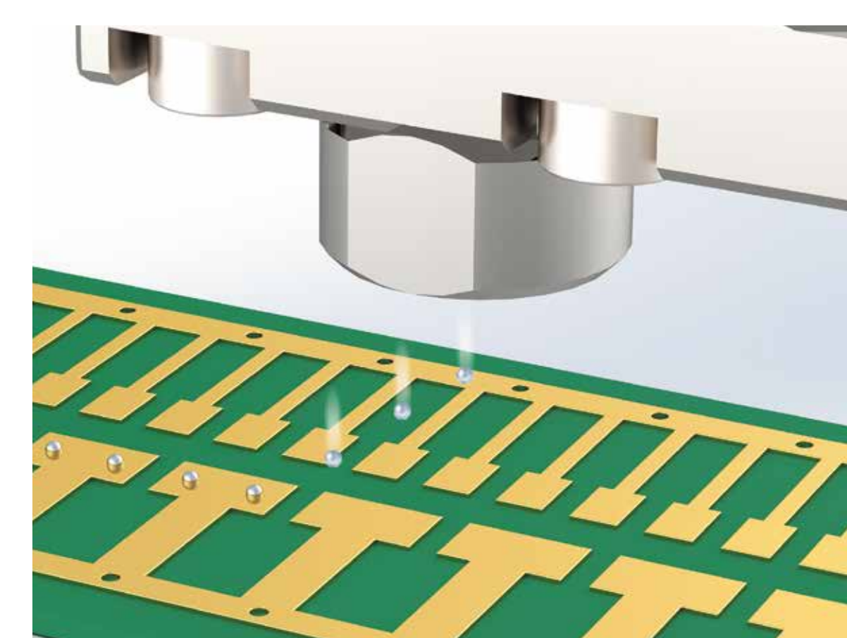
Ag dispensing on semiconductor lead frame
